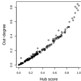
Hub Score and Out-Degree of Diplomatic Network
