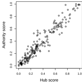
Hub and Authority Scores of Diplomatic Network
