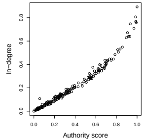
Authority Score and In-Degree of Diplomatic Network
